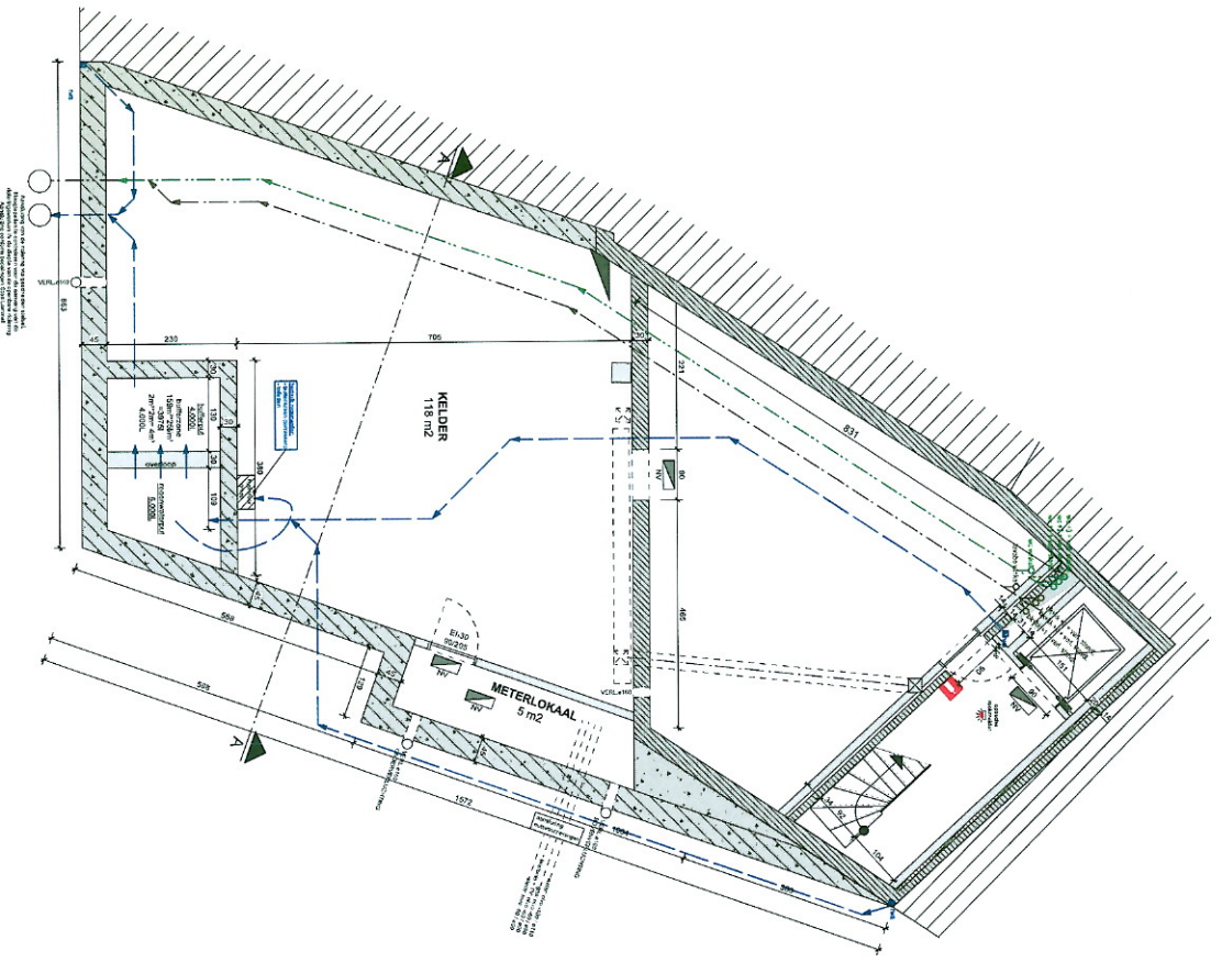
Fundering-Riolering 1:100
